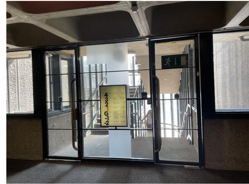
Example of steel door to stair towers within screen, with continuity of glazing bars, as proposed door D01
